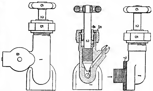
Figs. 3125-3126. CARBURETOR FILLING-VALVE.
